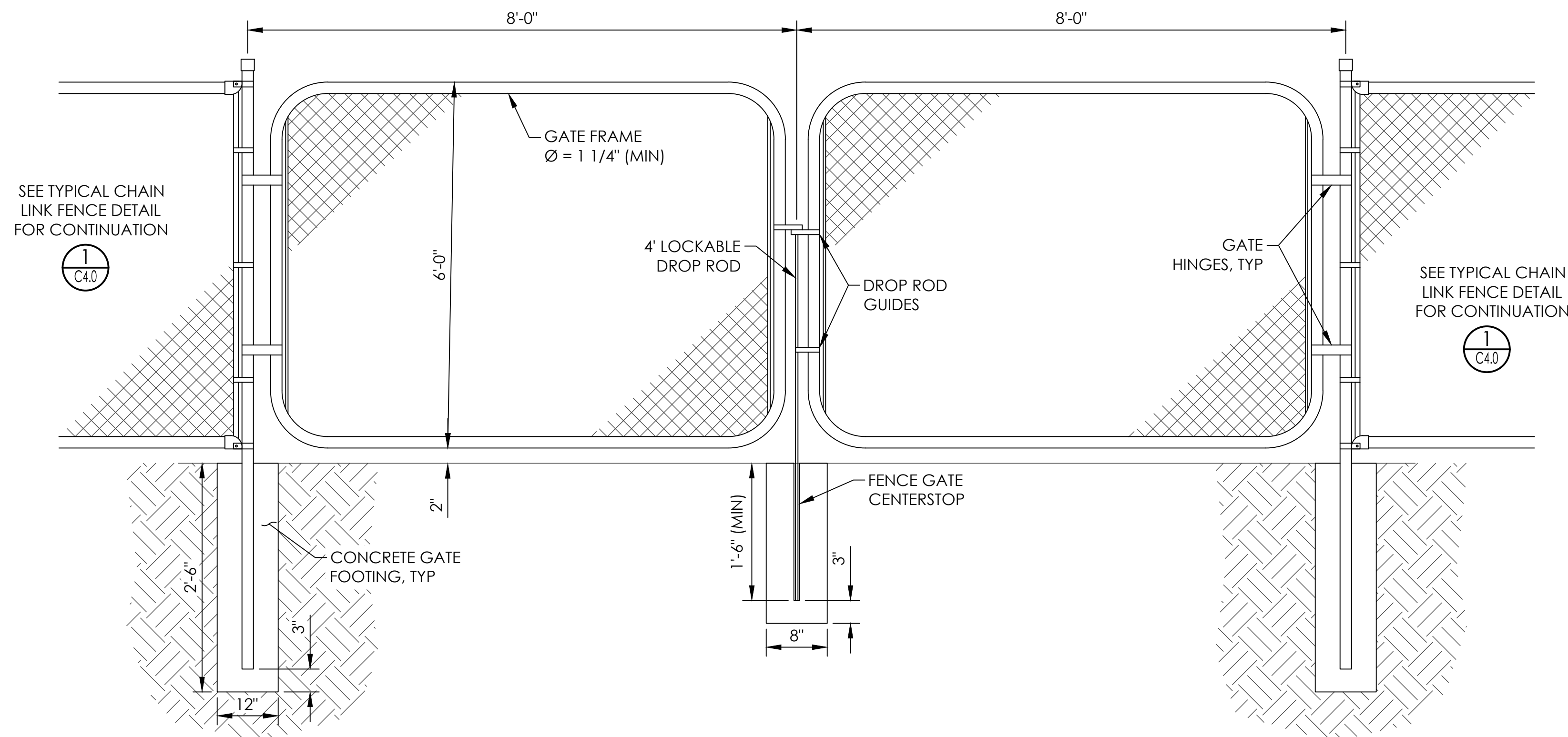
DRIVABLE GATE DETAIL NTS (4) C4.0
