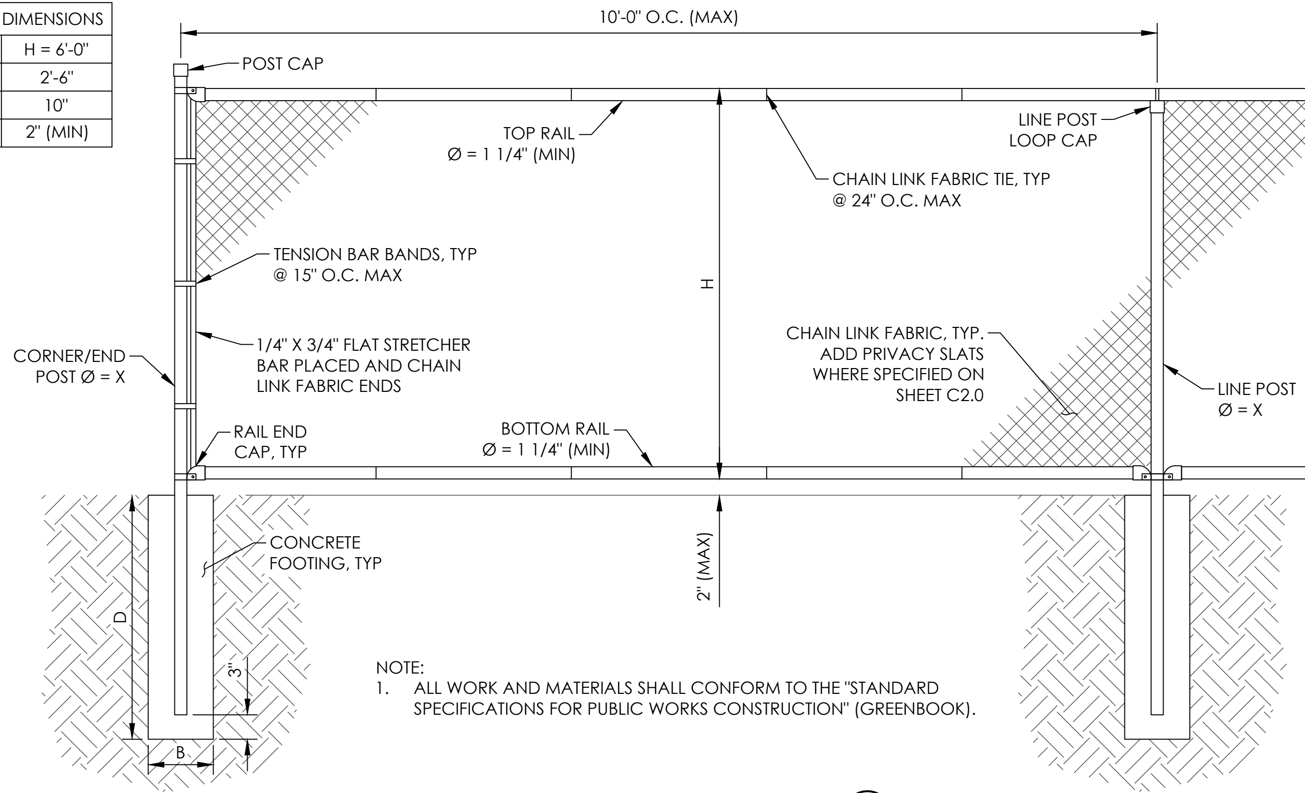
TYPICAL CHAIN LINK FENCE DETAIL NTS (1) C4.0
