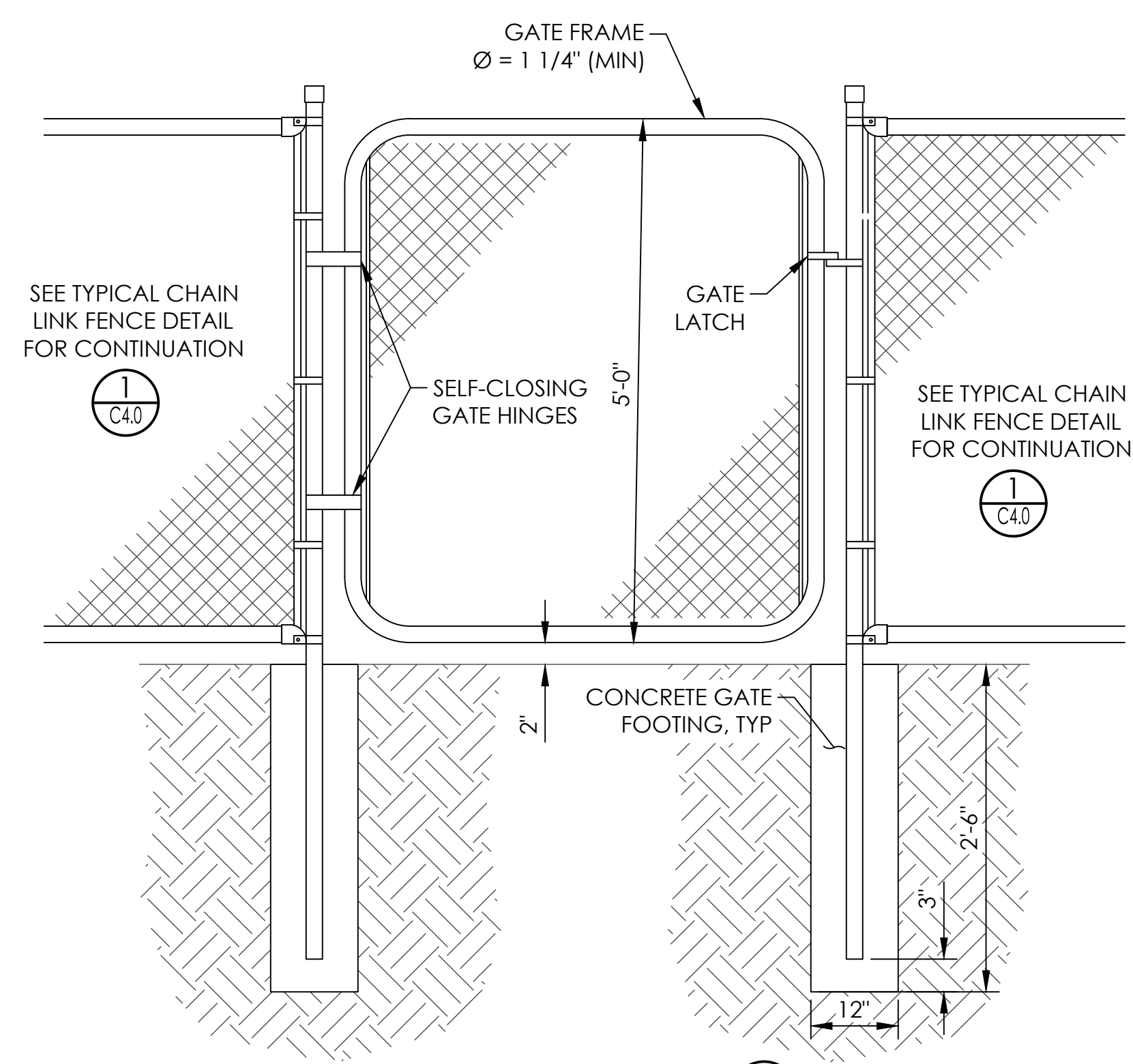
ENTRANCE GATE DETAIL NTS (2) C4.0
